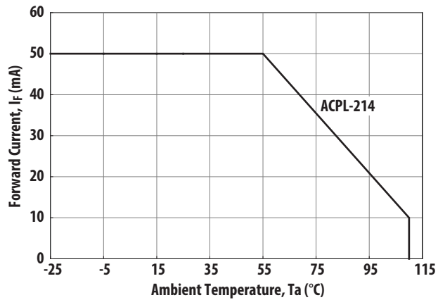
Figure 3 Forward Current vs. Ambient Temperature
