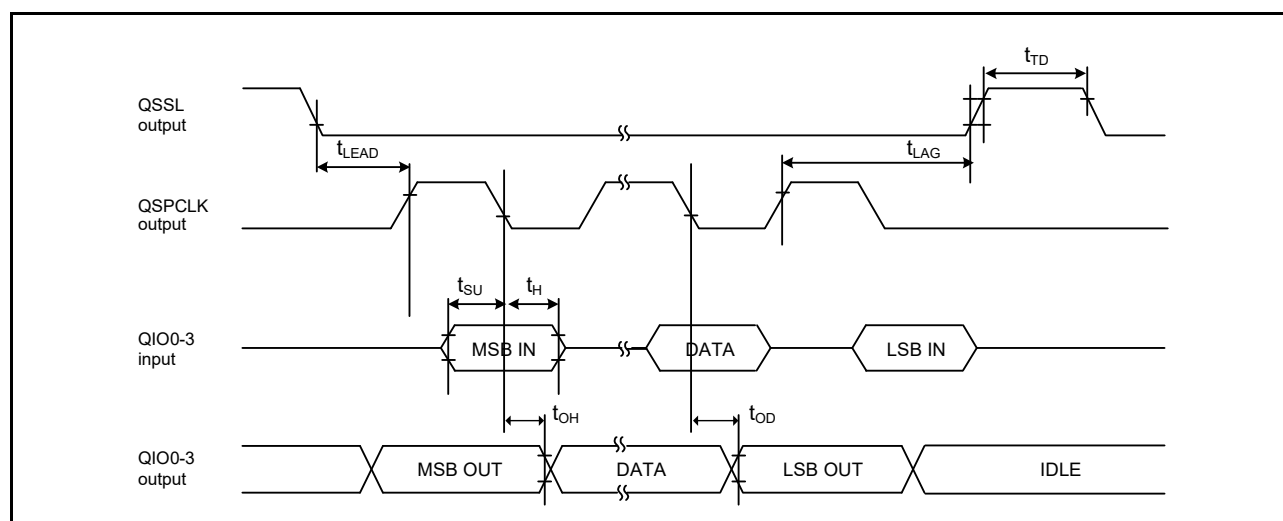
Figure 2.53 Transmit and receive timing
