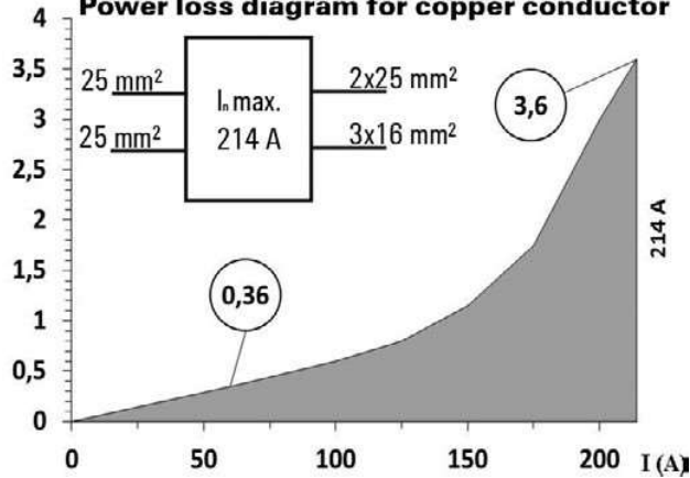
P (W) WPD x05 Power loss diagram for copper conductor
