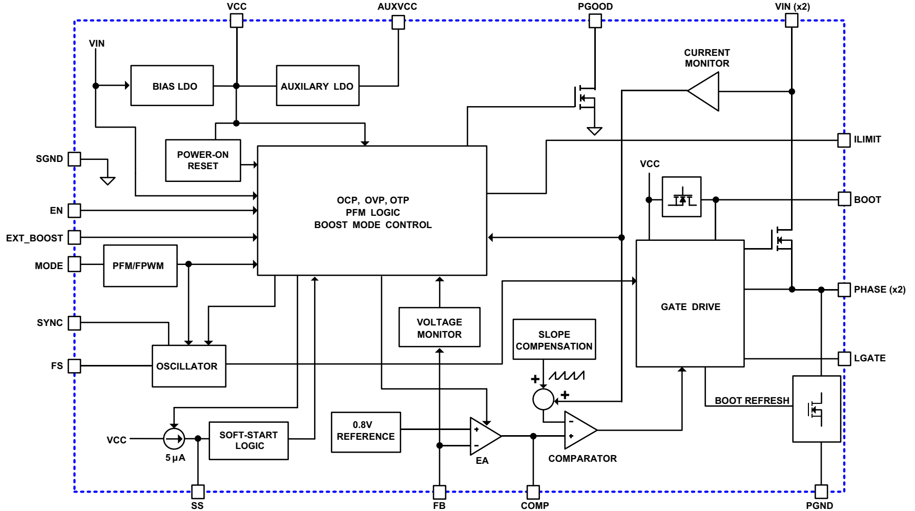
FIGURE 6. BLOCK DIAGRAM
