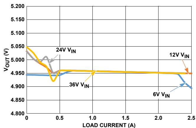
FIGURE 10. LOAD REGULATION, V_{OUT} 5V, T_A = +25°C
