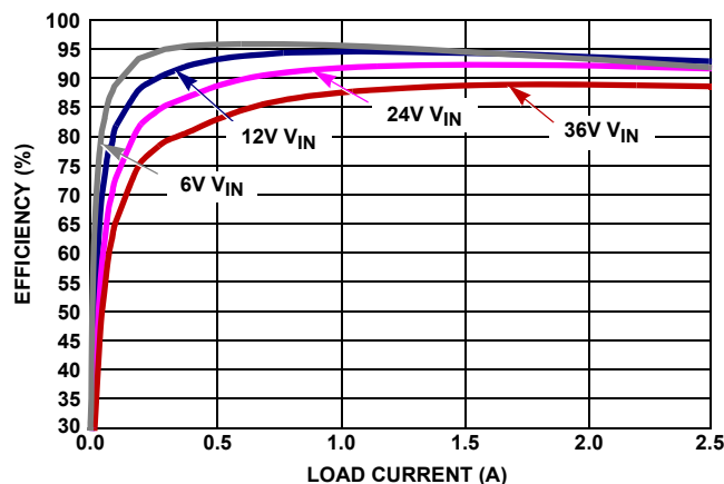
FIGURE 7. EFFICIENCY, SYNCHRONOUS BUCK, FORCED PWM MODE, 500kHz, V_{OUT} 5V, T_A = +25°C
