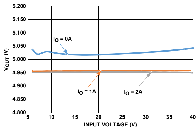
FIGURE 9. LINE REGULATION, V_{OUT} 5V, T_A = +25°C
