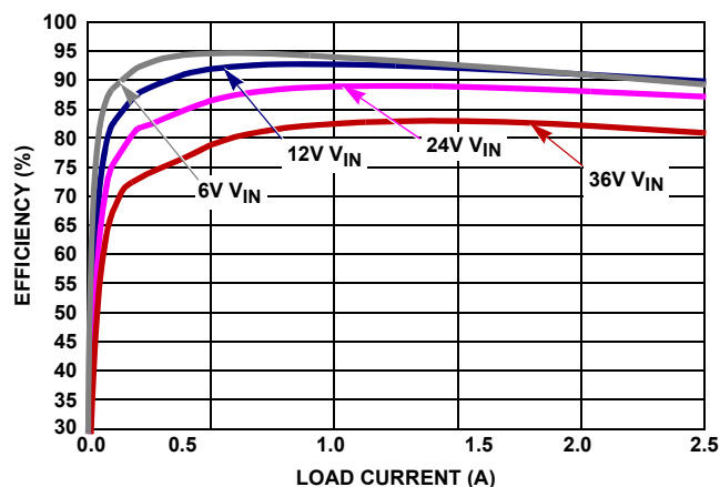
FIGURE 11. EFFICIENCY, SYNCHRONOUS BUCK, FORCED PWM MODE, 500kHz, V_{OUT} 3.3V, T_A = +25°C
