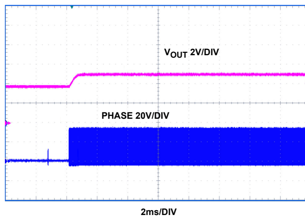
FIGURE 16. V_{IN} 36V , PREBIASED START-UP
