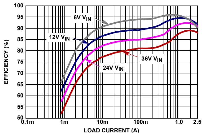
FIGURE 8. EFFICIENCY, SYNCHRONOUS BUCK, PFM MODE, V_{OUT} 5V, T_A = +25°C
