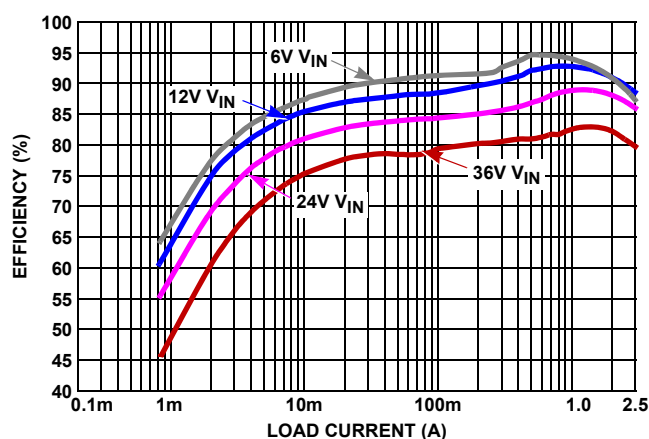
FIGURE 12. EFFICIENCY, SYNCHRONOUS BUCK, PFM MODE, V_{OUT} 3.3V, T_A = +25°C
