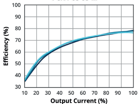
EFFICIENCY VS OUTPUT LOAD PCN1-S5-S5-M
