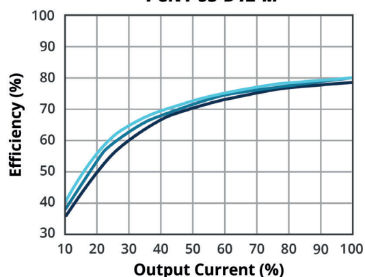
EFFICIENCY VS OUTPUT LOAD PCN1-S5-D12-M
