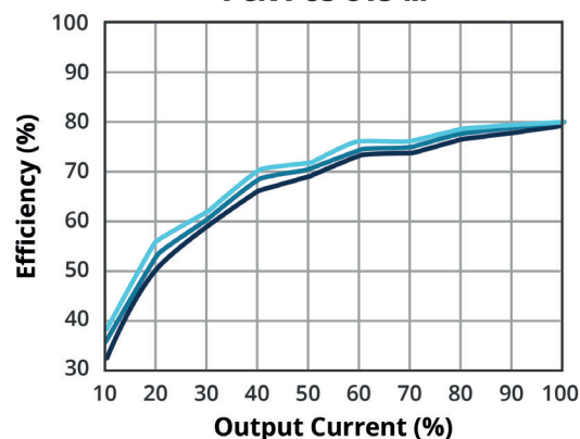
EFFICIENCY VS OUTPUT LOAD PCN1-S5-S15-M
