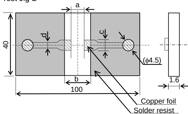
(2) Test Jig B
