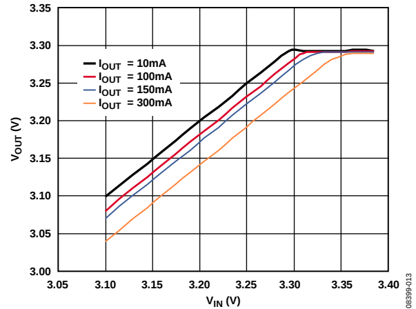
Figure 18. Output Voltage vs. Input Voltage (in Dropout)
