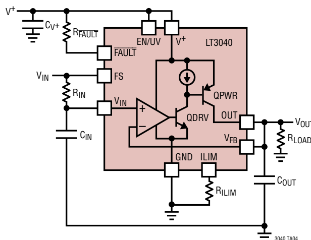
Figure 4. C_{IN} and C_{OUT} Connections for Stability
