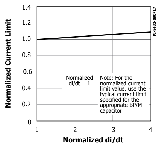
39. Standard Current Limit vs. di/dt .
