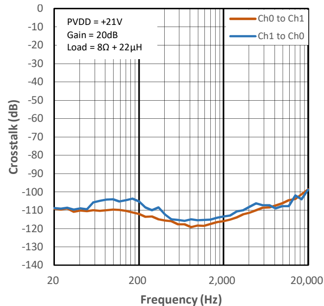
Figure 15-32 Crosstalk vs Frequency for PMP4
