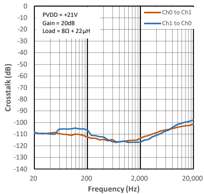
Figure 15-30 Crosstalk vs Frequency for PMP1
