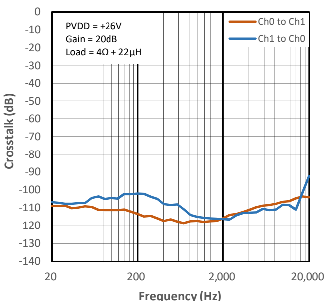
Figure 11-36 Crosstalk vs Frequency for PMP4
