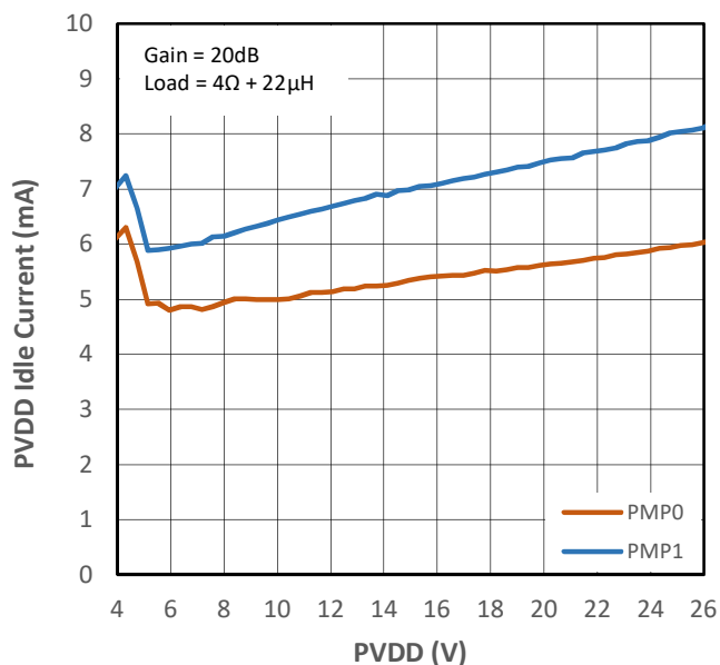
Figure 10-19 PVDD Idle Current vs PVDD for PMP0 & PMP1
