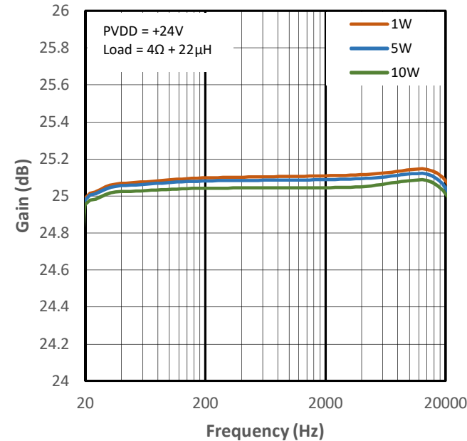
Figure 12-28 High Gain vs Frequency for PMP4
