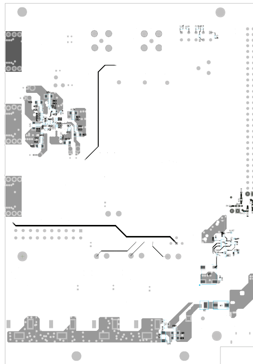
Figure 3-8: Layer 8 (BOT)
