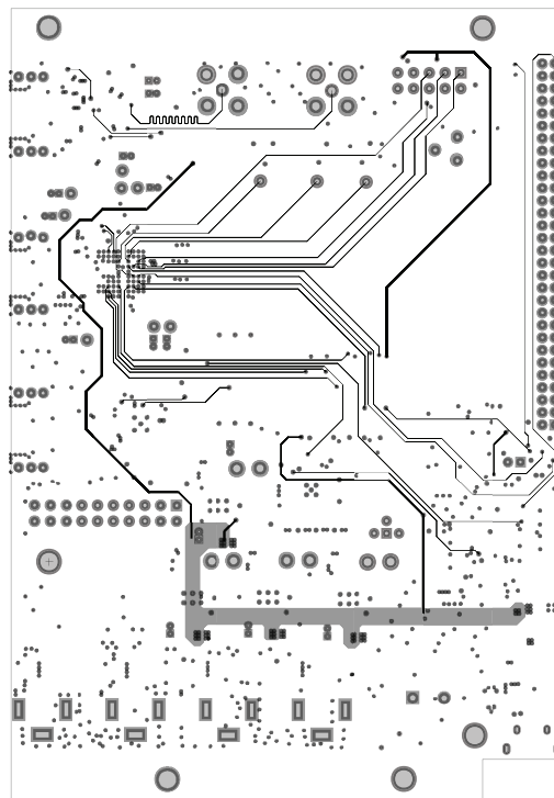
Figure 3-6: Layer 6 (SIG2)
