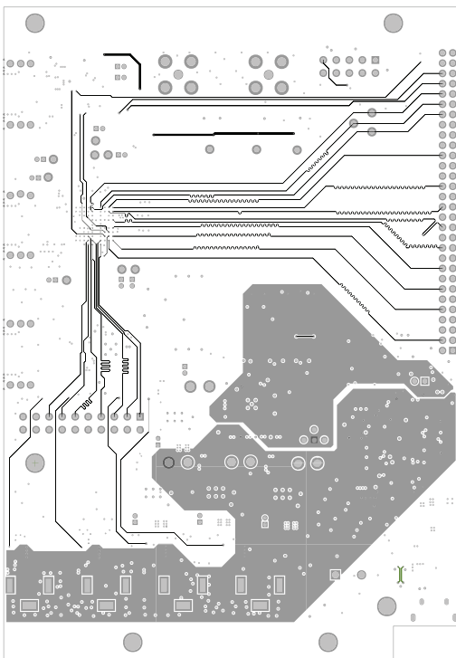
Figure 3-5: Layer 5 (SIG1)
