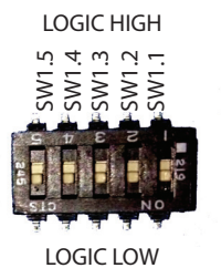
Figure 1-2: GS3471 Switch Configuration
