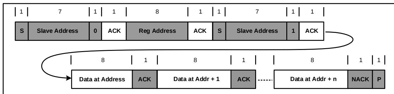
Figure 14: Multi-Read Sequence
