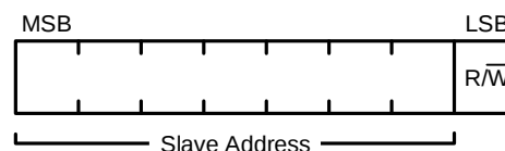
Figure 9: 7-Bit Addressing
