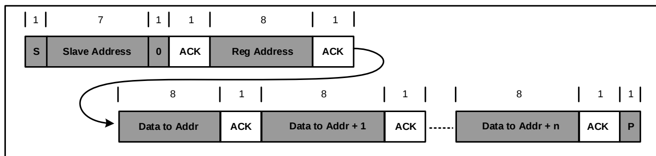
Figure 13: Multi-Write Sequence
