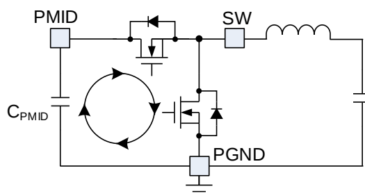
Figure 15: High-Frequency Current Path
