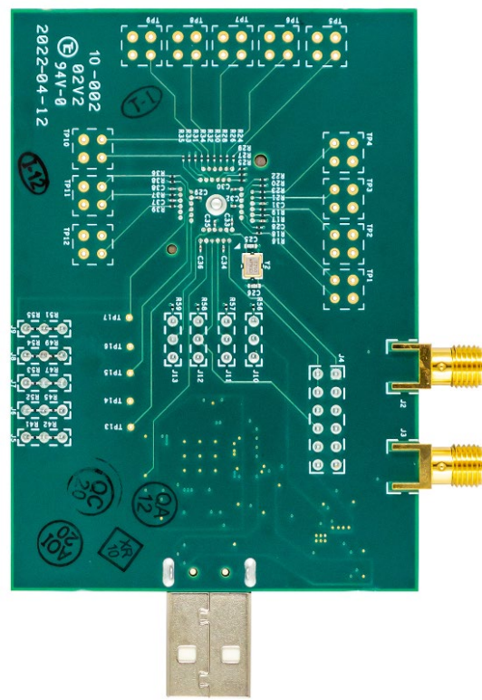
Figure 16. RC21012A/RC31012A Evaluation Board (Bottom)
