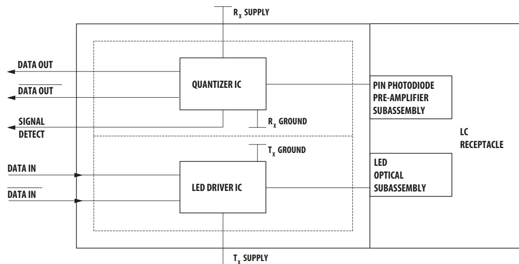
Figure 1: Block Diagram
