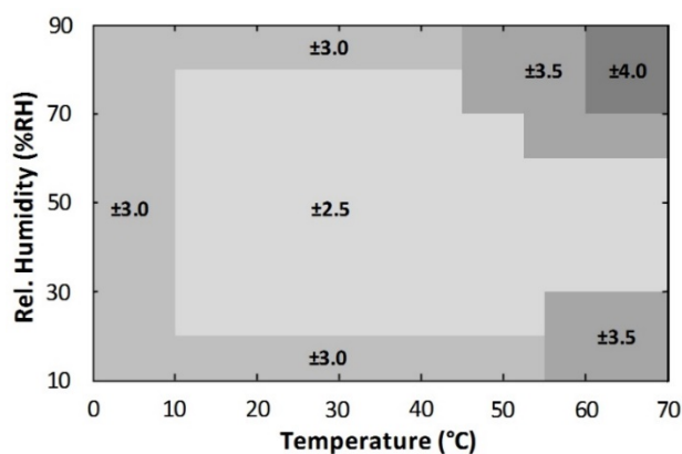
Figure 4. HS4113 RH Accuracy over Temperature
