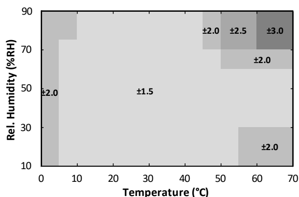
Figure 2. HS4111 RH Accuracy over Temperature
