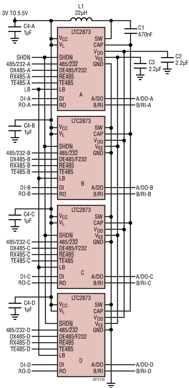
Figure 32. Quad Transceiver
