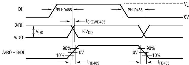
Figure 4. RS485 Driver Timing Measurement
