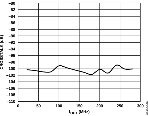
Figure 39. Crosstalk (DAC Set 1 to DAC Set 2), 4 \times Interpolation, f_{DATA} = 150 MSPS, Digital Scale = 0 dBFS, Full-Scale Current = 20 mA
