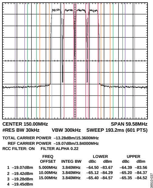
Figure 37. Four-Carrier W-CDMA, f_{OUT} = 150 MHz, f_{DAC} = 737.28 MSPS, 4 \times Interpolation, -3 dBFS, PLL On
