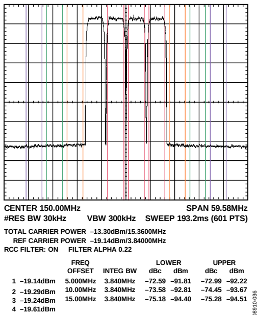
Figure 36. Four-Carrier W-CDMA, f_{OUT} = 150 MHz, f_{DAC} = 737.28 MSPS, 4 \times Interpolation, -3 dBFS, PLL Off
