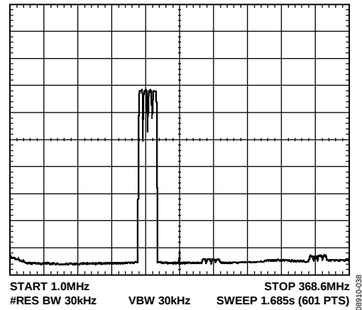
Figure 38. Four-Carrier W-CDMA, f_{OUT} = 150 MHz, f_{DAC} = 737.28 MSPS, 4 \times Interpolation, -3 dBFS
