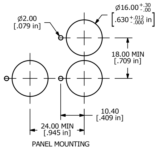
PANEL MOUNTING
