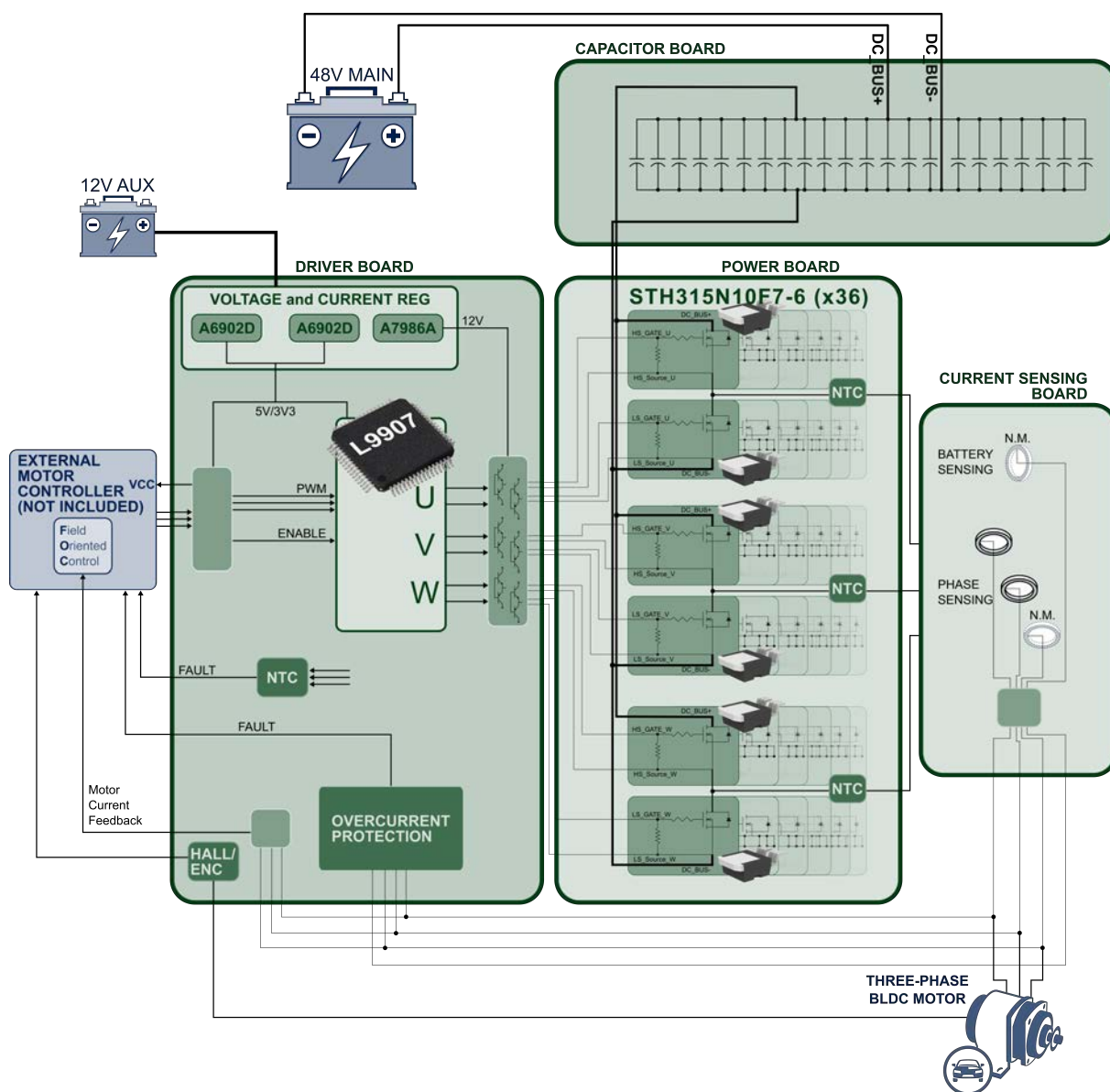
Figure 1. Block diagram for automotive motor control applications
