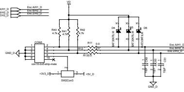
Figure 5. Driver board schematics - sensing and status
