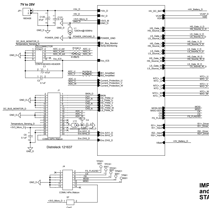
Figure 4. Driver board schematics - main with connectors
