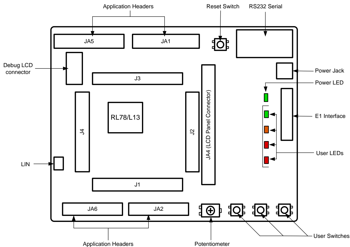
Figure 3-1: Board Layout
