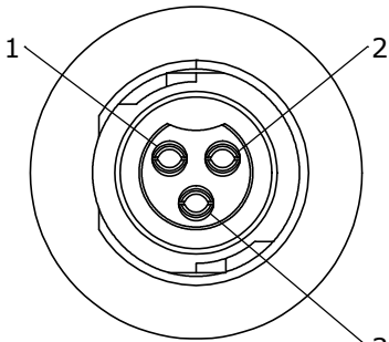
FACE VIEW W17282-3SG-P-300
