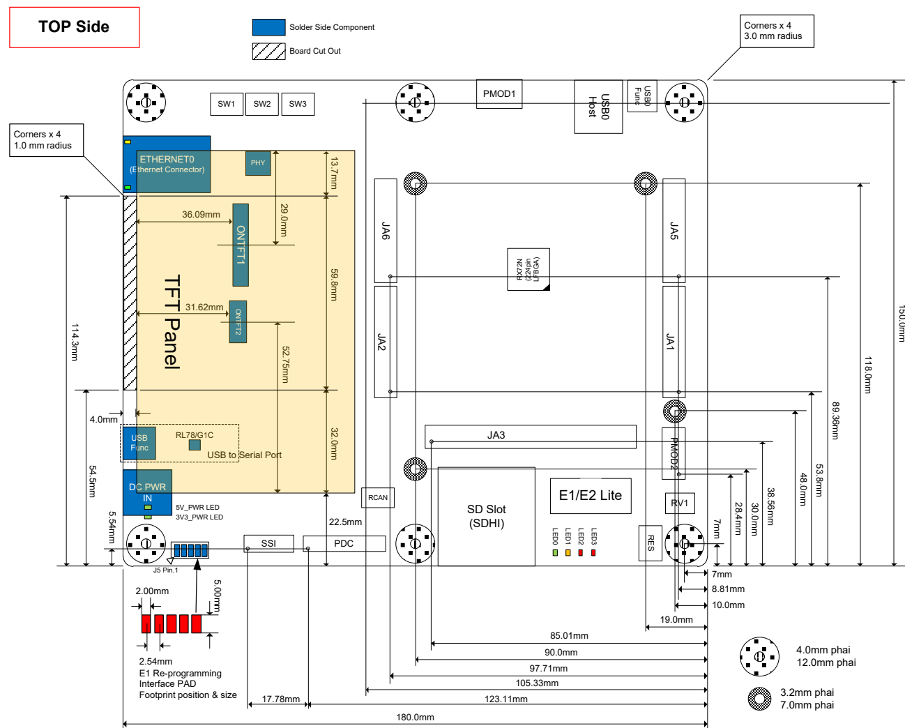
Figure 3-2: Board Dimensions
