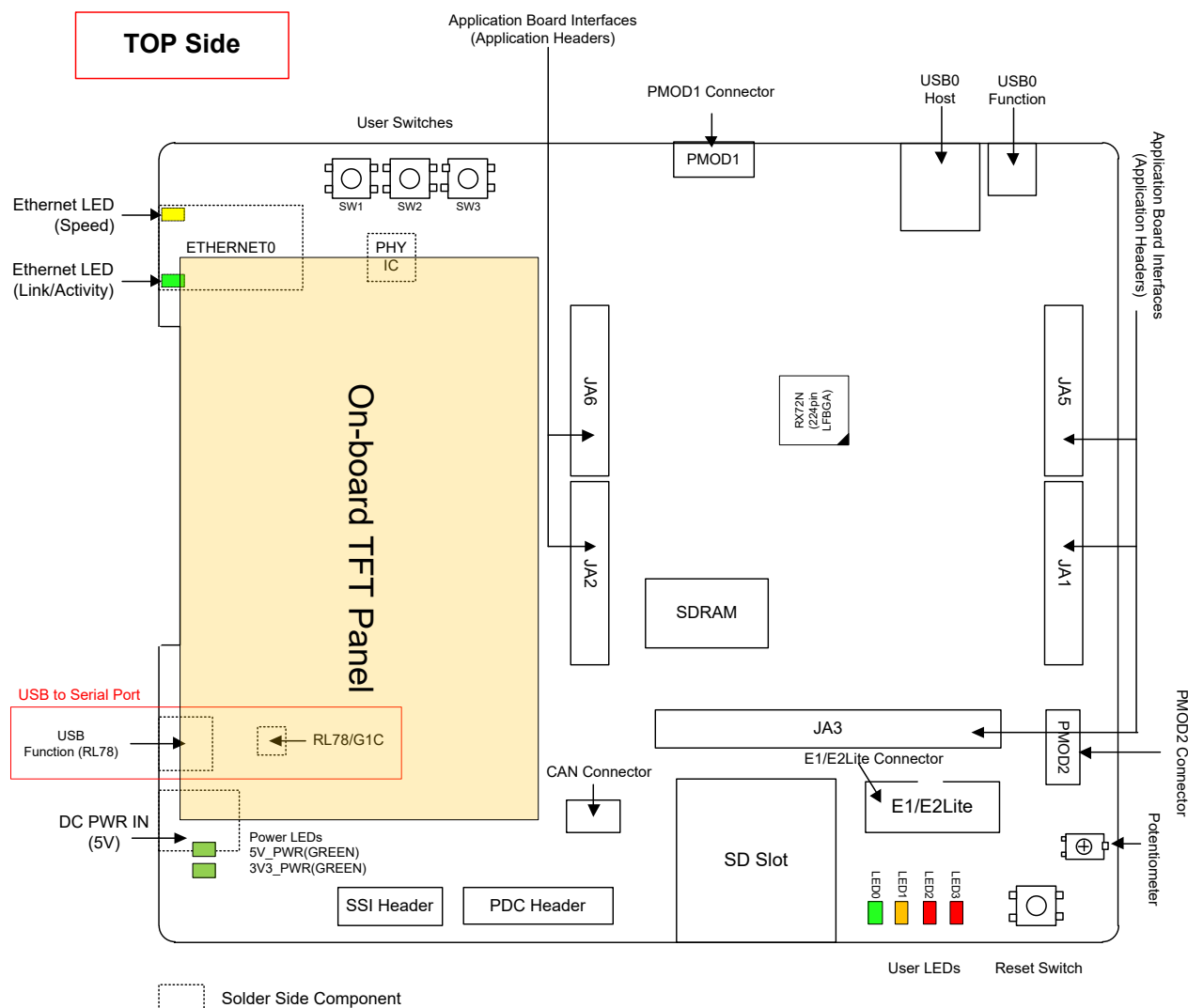
Figure 3-1: Board Layout
