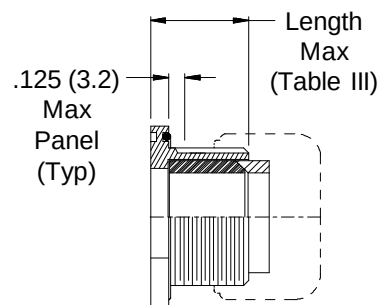
Style 2 - Environmental Type A - Rear Mount
