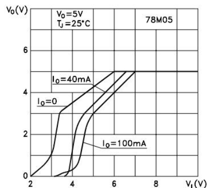
Figure 9. Dropout characteristics
