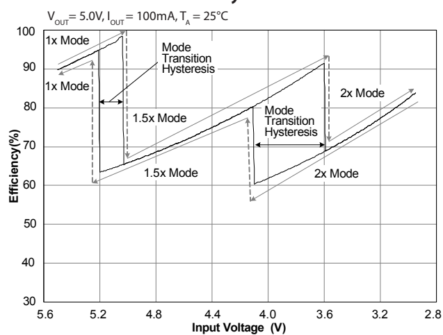
Efficiency — 100mA
