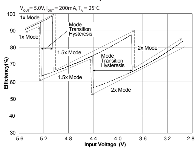
Efficiency — 200mA
