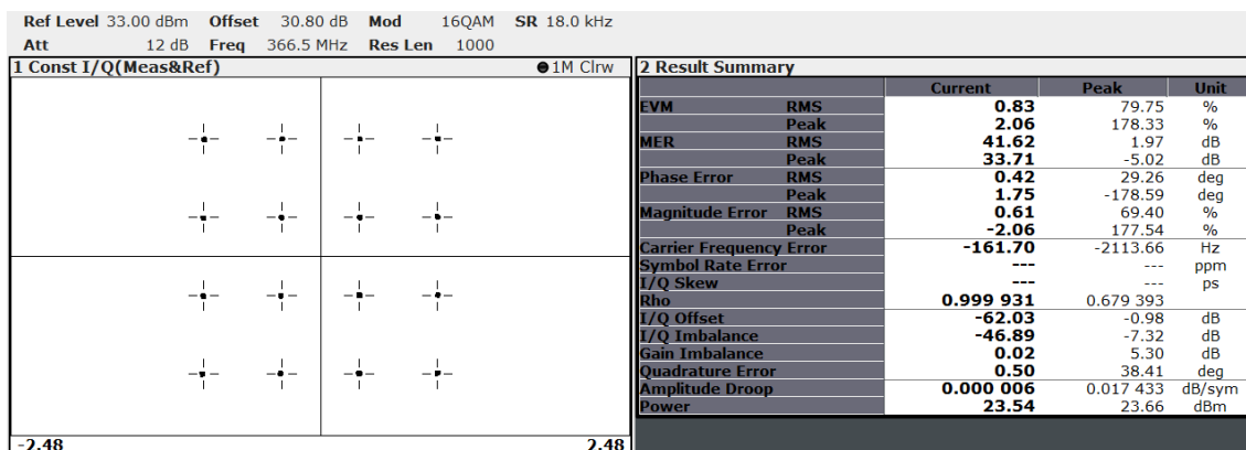
Figure 26 16-QAM, 18 ks/s, Constellation and EVM at 366.5MHz
