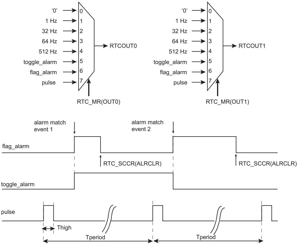
Figure 27-6. Waveform Generation
