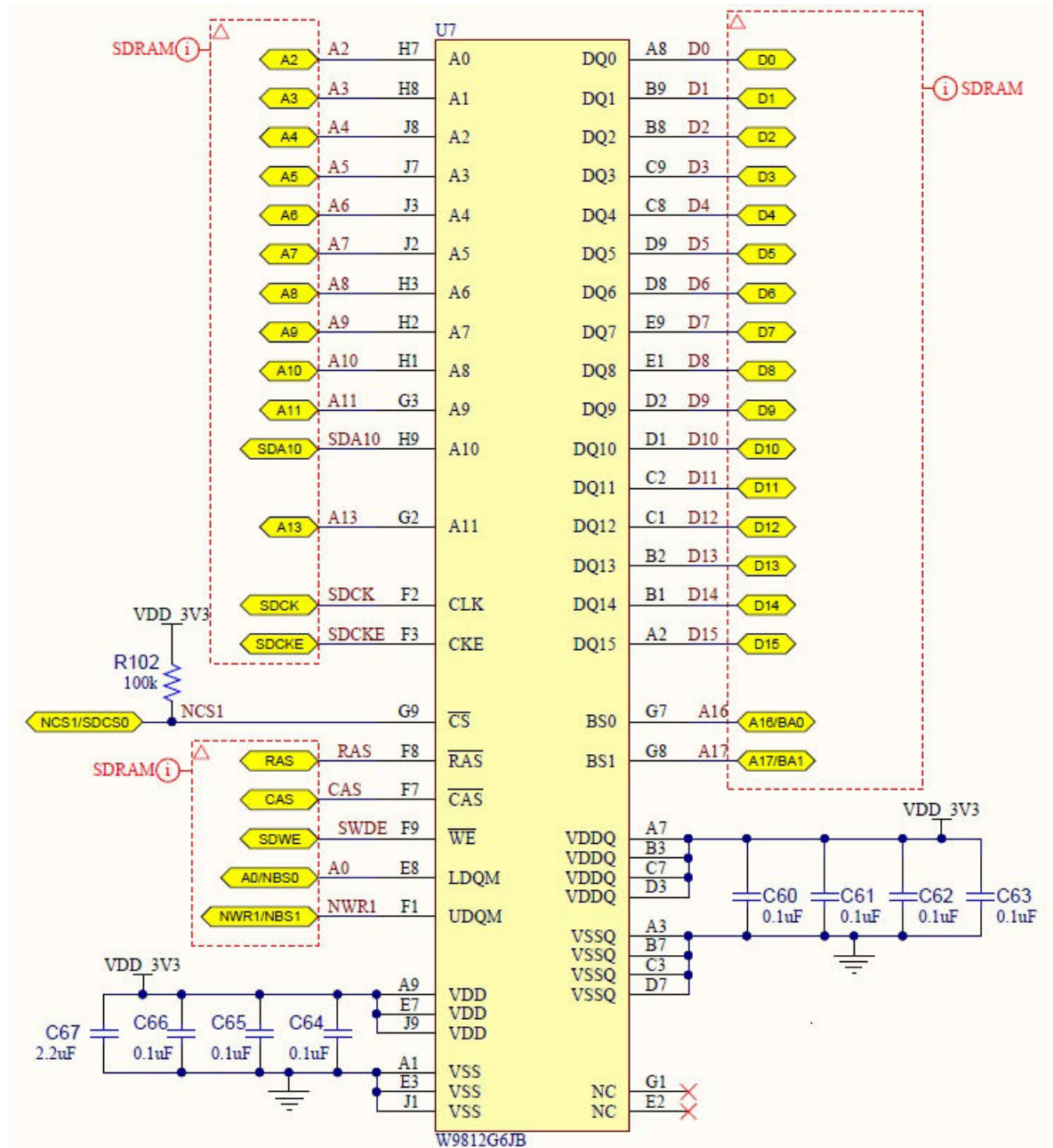
Figure 33-2. Hardware Configuration
