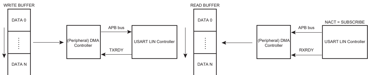
Figure 46-53. Client Node with DMAC
