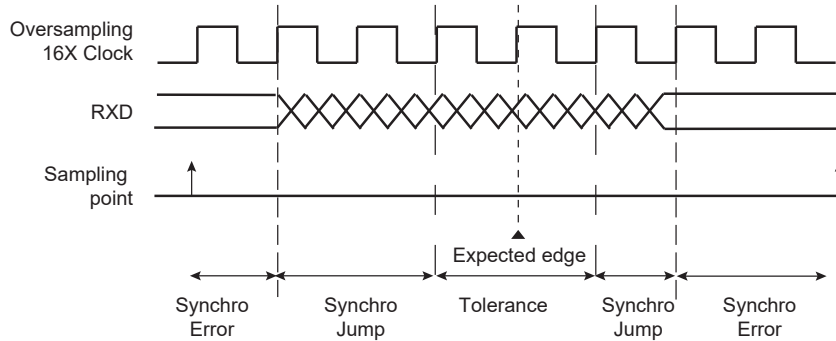
Figure 46-10. Bit Resynchronization
