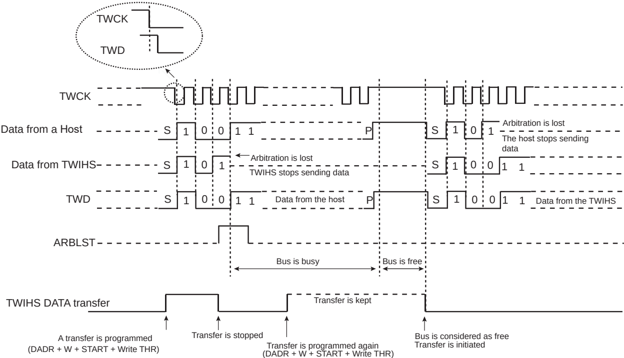
Figure 43-29. Arbitration Cases
