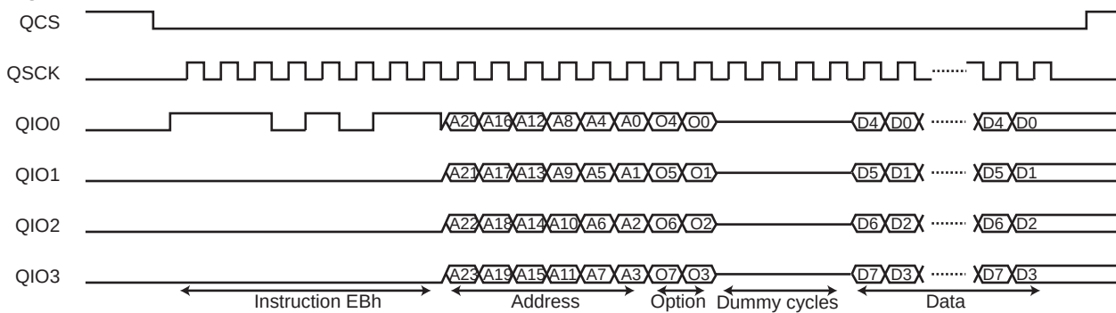
Figure 42-8. Instruction Frame
