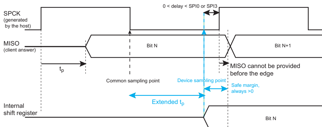
Figure 59-20. SPI Host Mode with (CPOL= NCPHA = 0) or (CPOL= NCPHA= 1)
