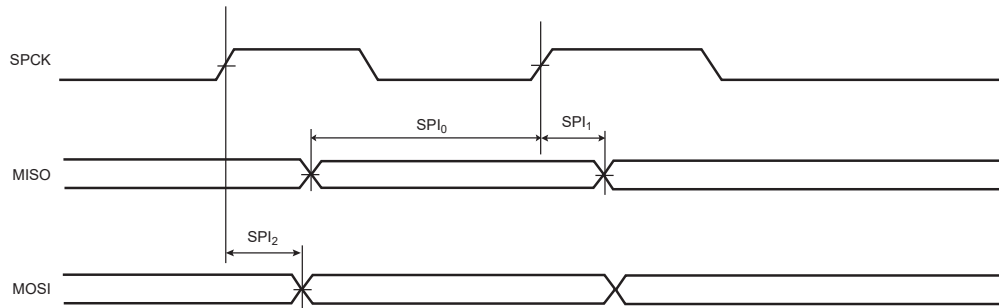
Figure 58-21. SPI Host Mode with (CPOL = 0 and NCPHA=1) or (CPOL=1 and NCPHA= 0)
