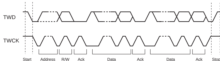
Figure 43-3. Transfer Format
