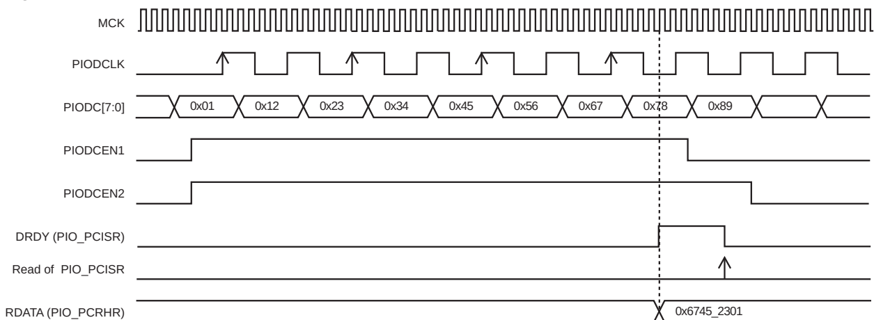
Figure 32-12. Parallel Capture Mode Waveforms (DSIZE = 2, ALWYS = 0, HALFS = 1, FRSTS = 0)
