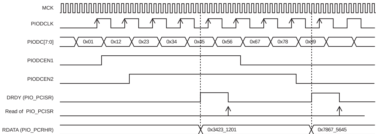
Figure 32-12. Parallel Capture Mode Waveforms (DSIZE = 2, ALWYS = 0, HALFS = 1, FRSTS = 0)
