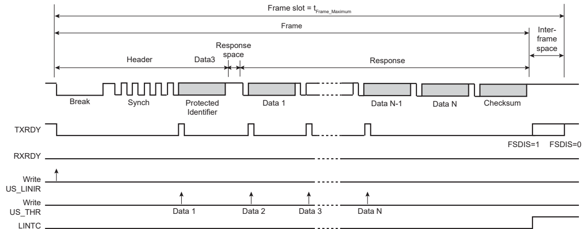
Figure 46-46. Host Node Configuration, NACT = SUBSCRIBE
