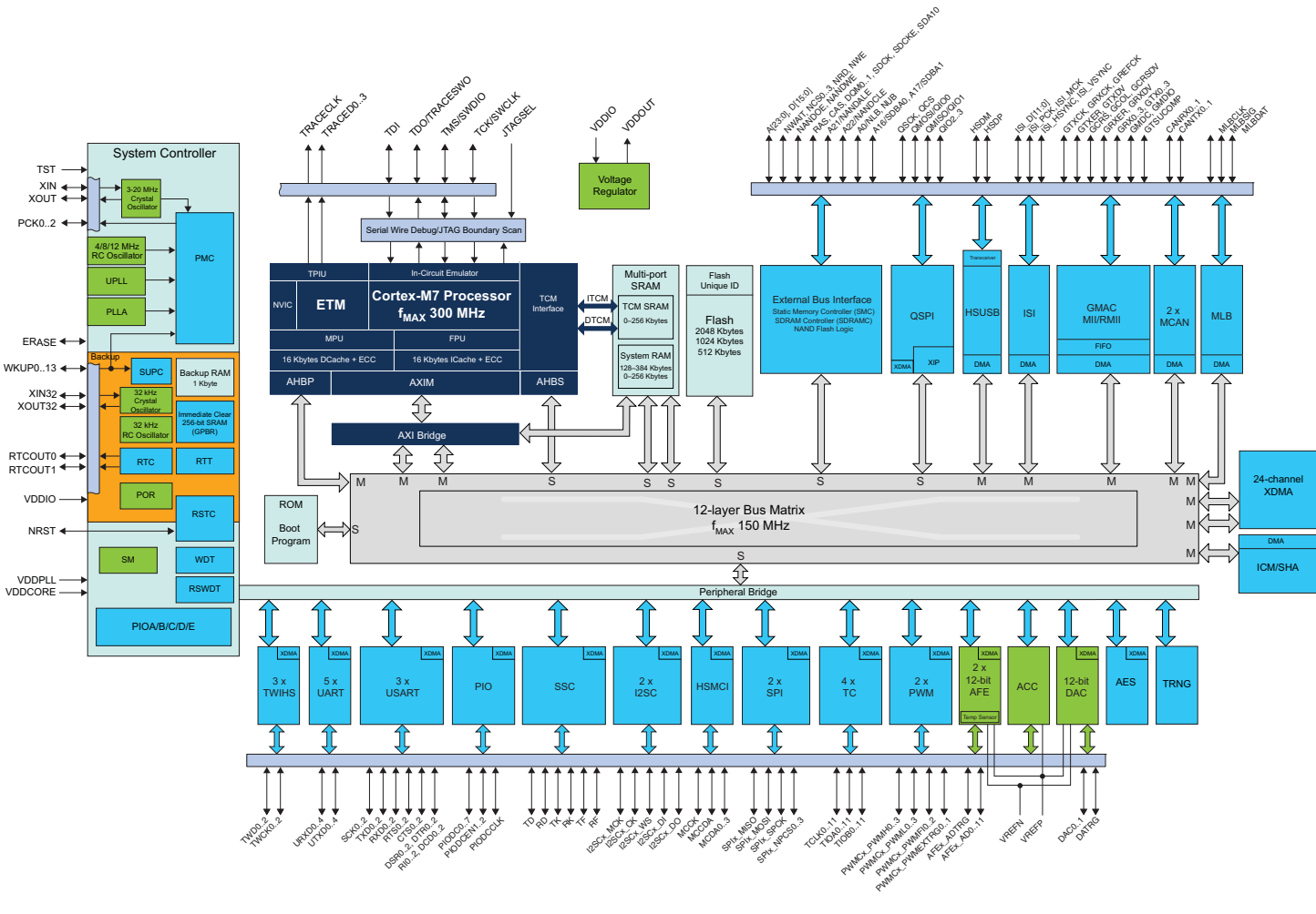
Figure 3-4. SAM V71 144-pin Block Diagram
