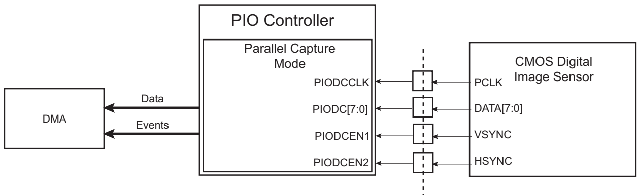
Figure 32-8. PIO Controller Connection with CMOS Digital Image Sensor
