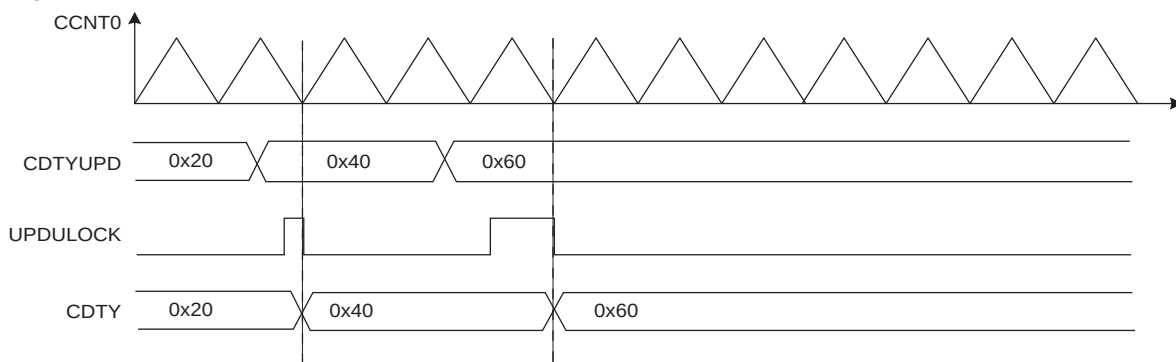
Figure 51-19. Method 1 (UPDM = 0)
