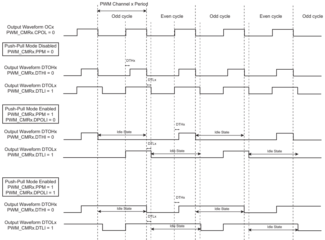
Figure 51-10. PWM Push-Pull Mode
