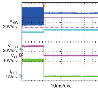
Short V_{OUT} to GND
