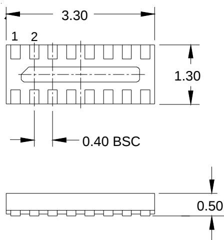
Nominal Dimensions in mm (Bottom View)
