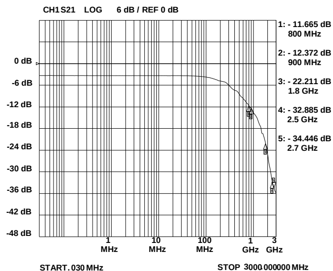
TLP Characteristic
