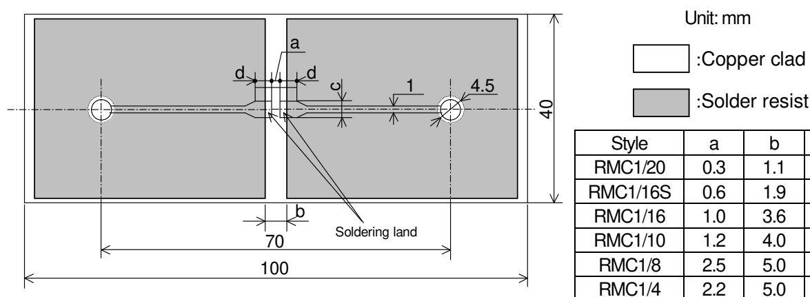
RMC1/20, 1/16S, 1/16, 1/10, 1/8, 1/4 BOUND STRENGTH OF THE END FACE PLATING TEST SUBSTRATE
