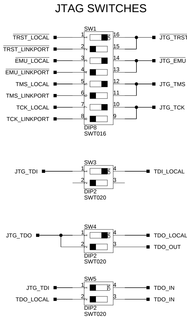
MULTI PROCESSOR JTAG SETTINGS VIA HP-USB EMULATOR USING TWO OR MORE EZ-BOARDS (LINK PORT CABLES REQUIRED FOR MORE THAN TWO BOARDS)
