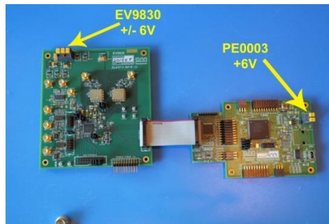
Figure 3: Power Supply Connections
