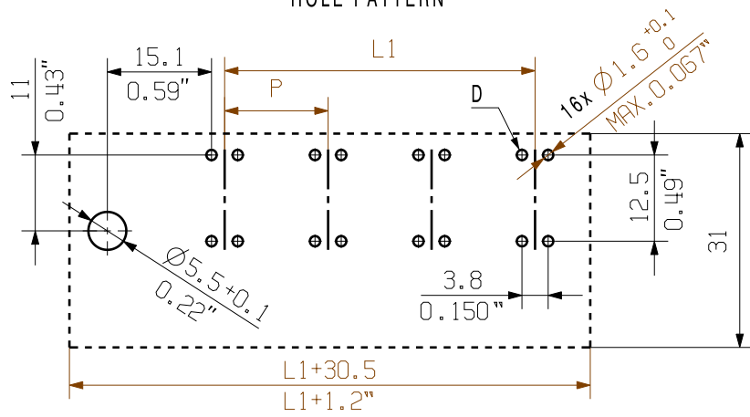
HOLE PATTERN
