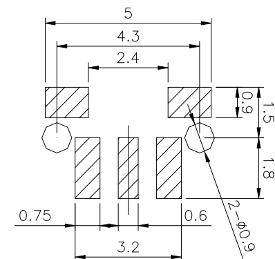
PCB. 焊接图 PCB. WELDING DRAWING
