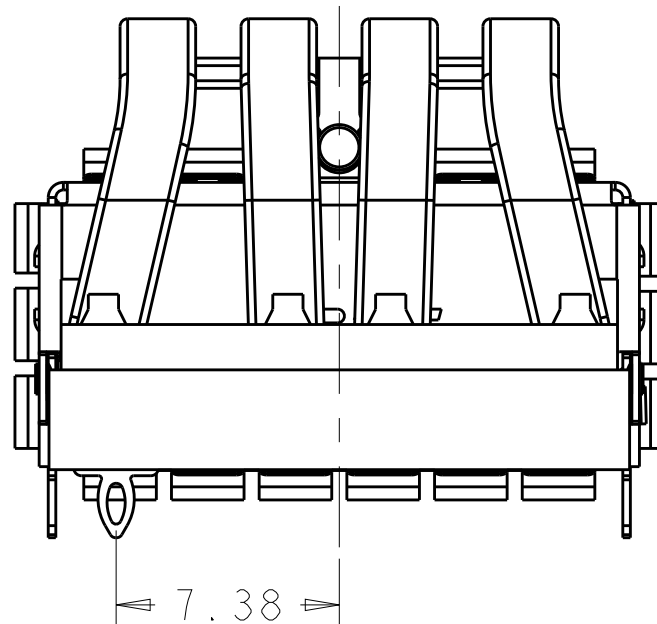
BACK VIEW OF 2170773-5 SCALE 4:1
