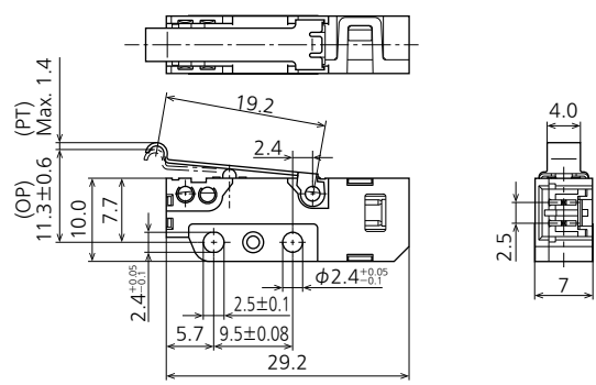
External dimensions
