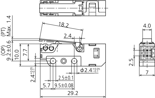
External dimensions
