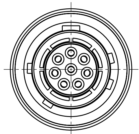
K11YCR-P08WFG0-0000 Mechanical coding: C Color coding: blue
