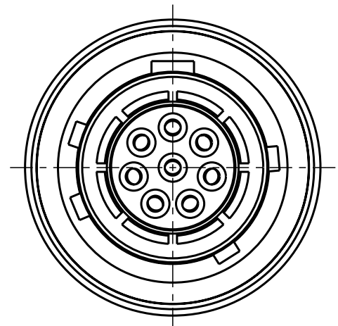
K11YDR-P08WFG0-0000 Mechanical coding: D Color coding: green
