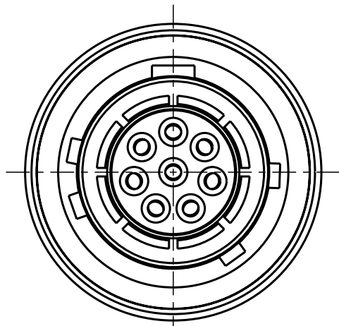
K11YBR-P08WFG0-0000 Mechanical coding: B Color coding: red
