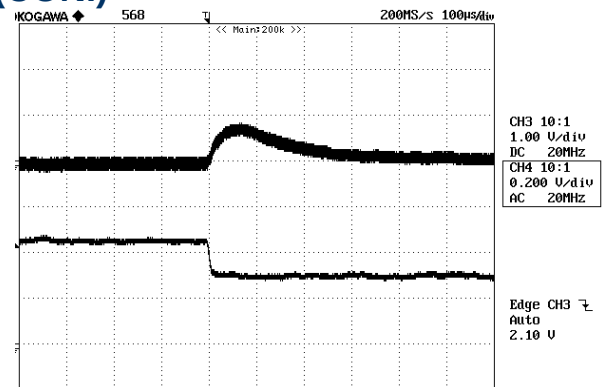
Figure 8: Output voltage response to step-change in load current (75%-50% of I_o , max; di/dt = 0.1A/\mu s ). Load cap: 10 \mu F tantalum capacitor and 1 \mu F ceramic capacitor. Top Trace: V_{out} (200mV/div, 100 \mu s /div), Bottom Trace: I_{out} (1A/div). Scope measurement should be made using a BNC cable (length shorter than 20 inches). Position the load between 51 mm to 76 mm (2 inches to 3 inches) from the module.
