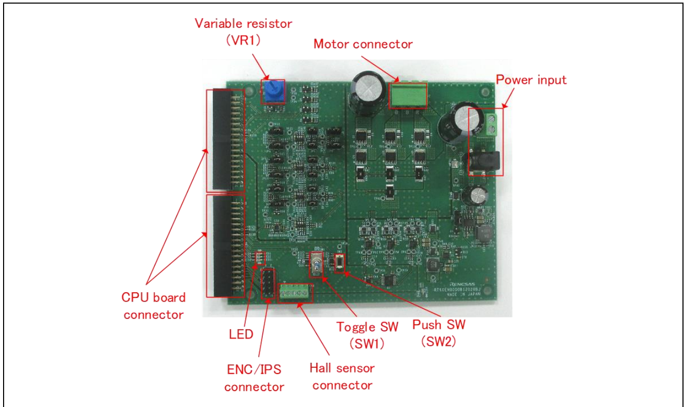
Figure 4-2 Inverter Board
