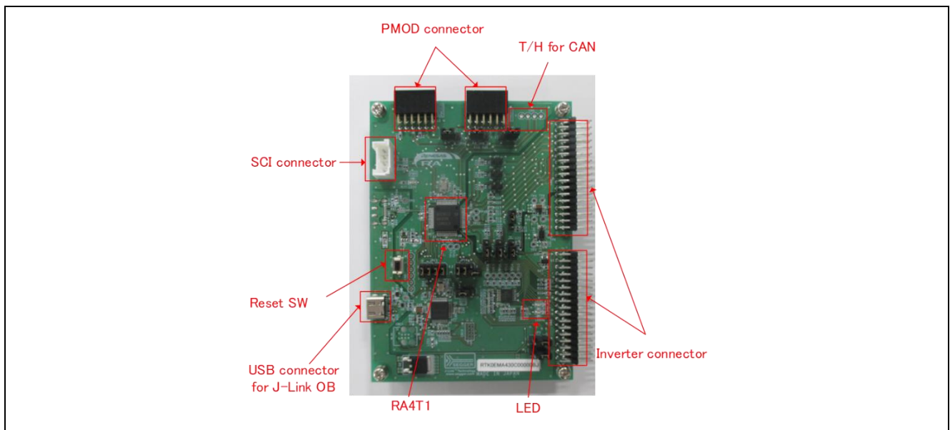
Figure 4-3 CPU Board
