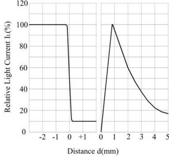
Fig.7 Sensing Position Characteristics (Typical)
