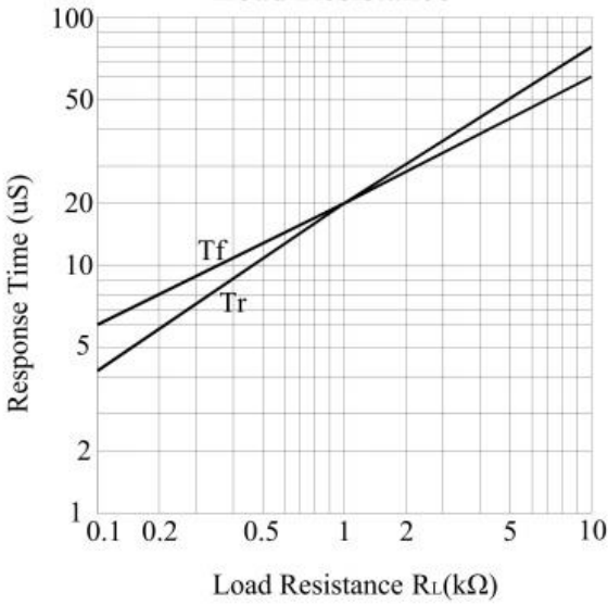
Fig.6 Response Time vs. Load Resistance
