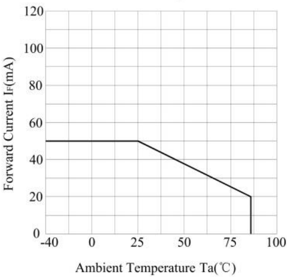
Fig.8 Forward Current Derating Curve vs. Ambient Temperature
