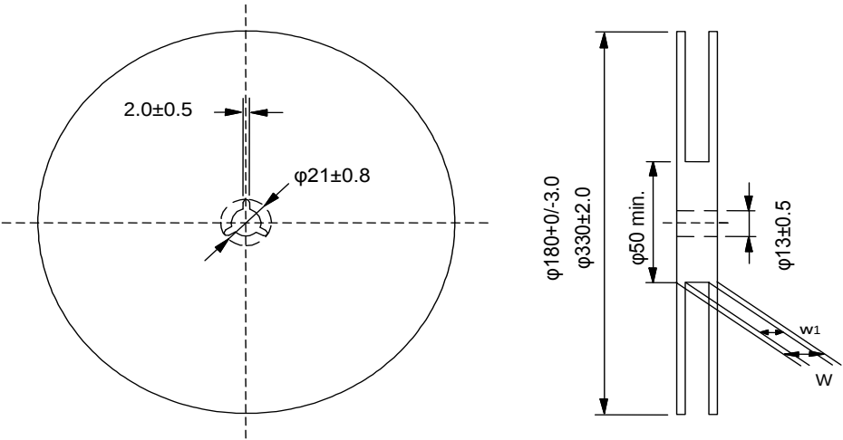
Fig.3 Taping Diagram
