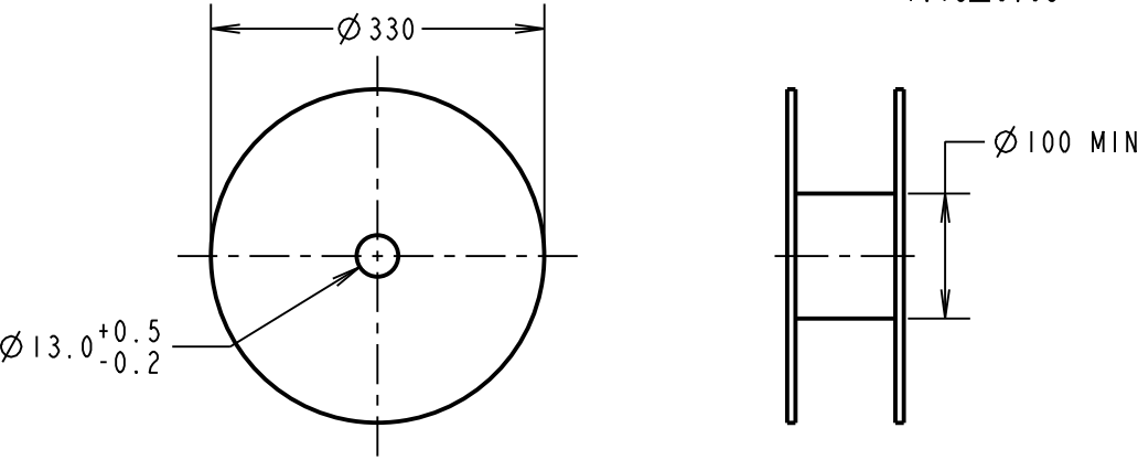
REEL DETAILS
