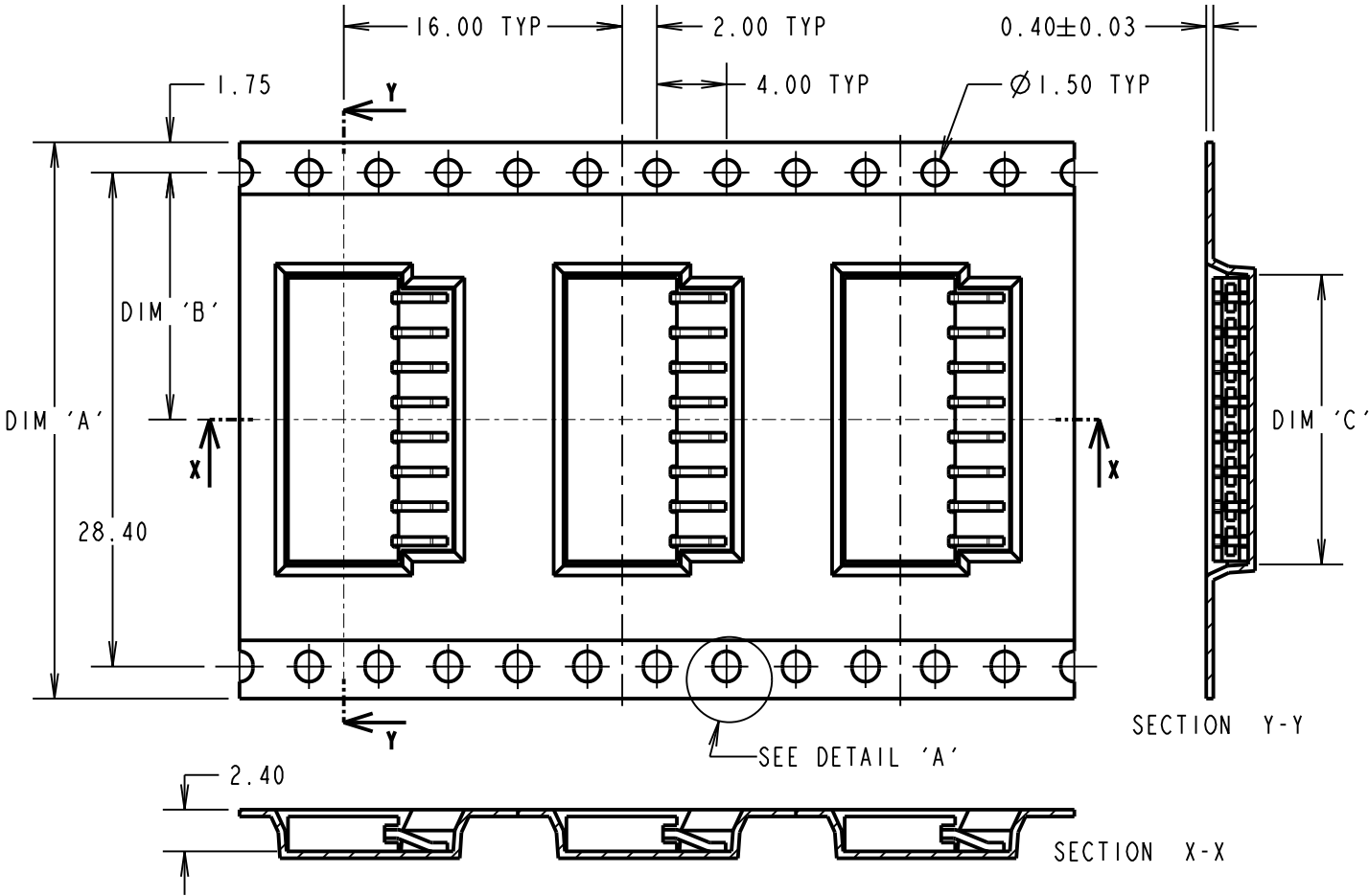
TAPE DETAILS FOR 08 & 10 WAY
