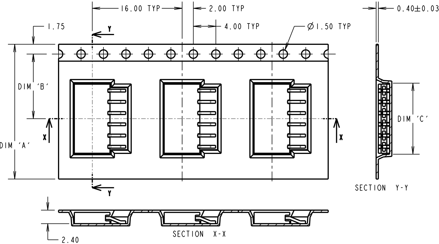
TAPE DETAILS FOR 02, 03, 04, 05 & 06 WAY
