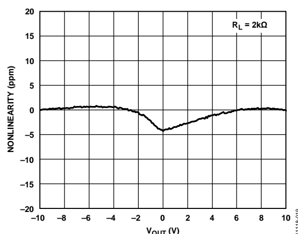
Figure 22. Gain Nonlinearity
