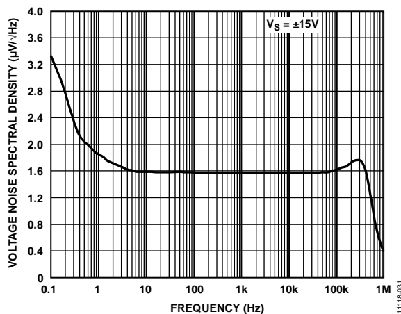
Figure 33. Voltage Noise Spectral Density vs. Frequency
