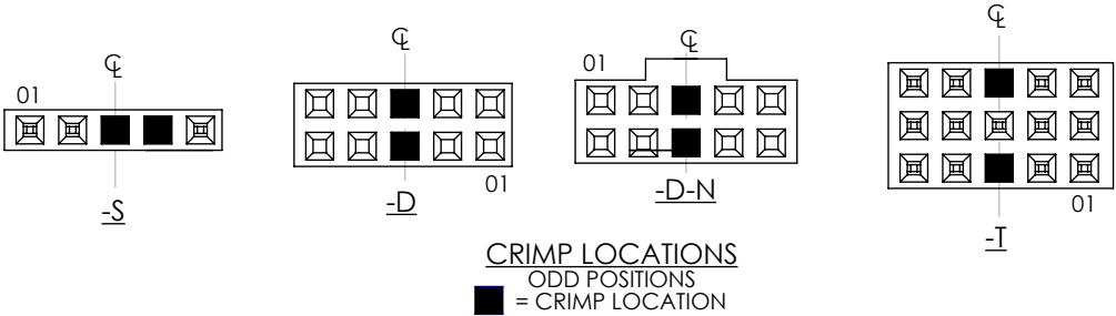
FIG 2 RIGHT ANGLE OPTION ALL OPTIONS DIFFERENT AS SHOWN, OTHERWISE SAME AS -S-RA
