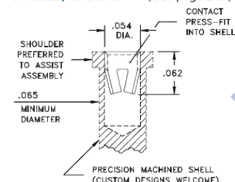
#18 CONTACT FOR .037"-.043" DIAMETER PINS ( \phi = .004 ) 6-FINGER, GROUP L (See page 248)
