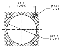
PERCAGE PANNEAU PANEL DRILLING
