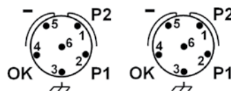
Pin-out for the 2 power connectors of the Ring and managed models Note: The use of 2 connectors facilitates the cabling of redundant power inputs.
