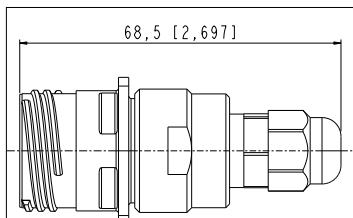
Backshell used with back termination type 2: Solder (Sealed – IP68)
