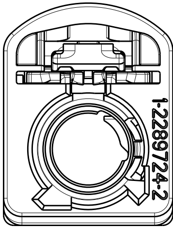
DETAIL M SCALE 4:1
