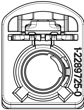
DETAIL K SCALE 4:1
