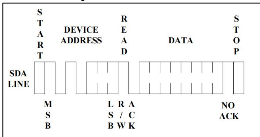
Figure 9. Random Read
