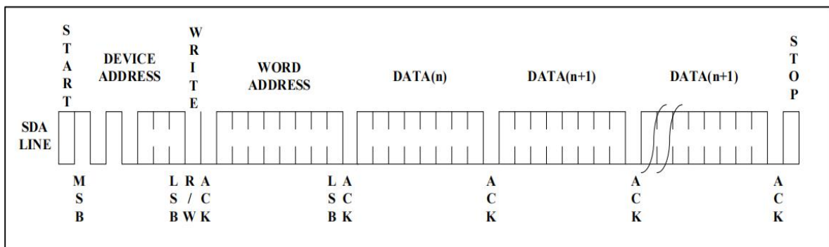
Figure 7. Page Write
