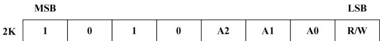
Figure 6. Byte Write
