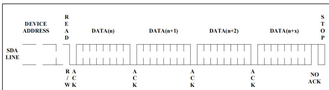
Figure 10. Sequential Read
