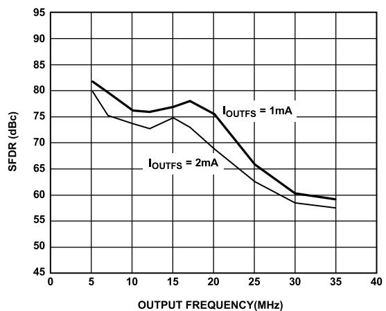
Figure 31. SFDR vs. f_{OUT} and I_{OUTFS} at 80 MSPS
