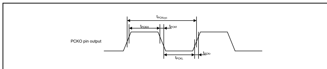
Figure 2.96 PDC Output Clock Timing
